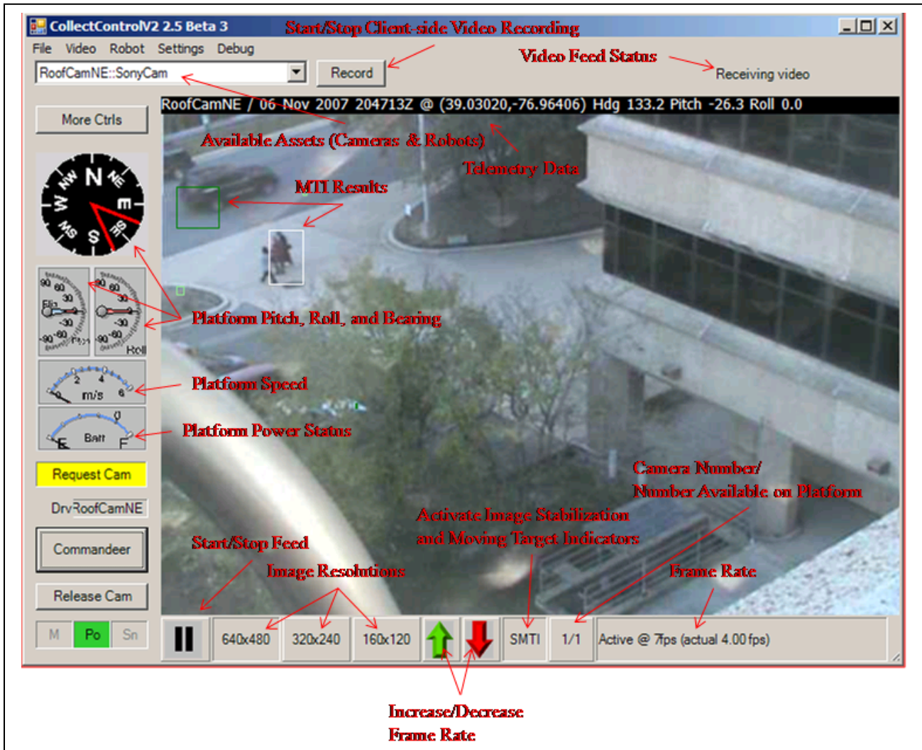
Figure 12. ARL UGV OCU C2 application.
